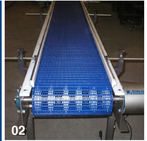
MODULAR CONVEYOR
